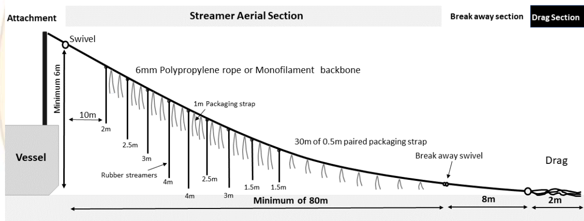
Figure 1. A schematic representation of bird-scaring line design for vessels UNDER 35m , with streamers and a drag
